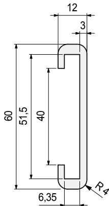
Guide rail (extra flat)
