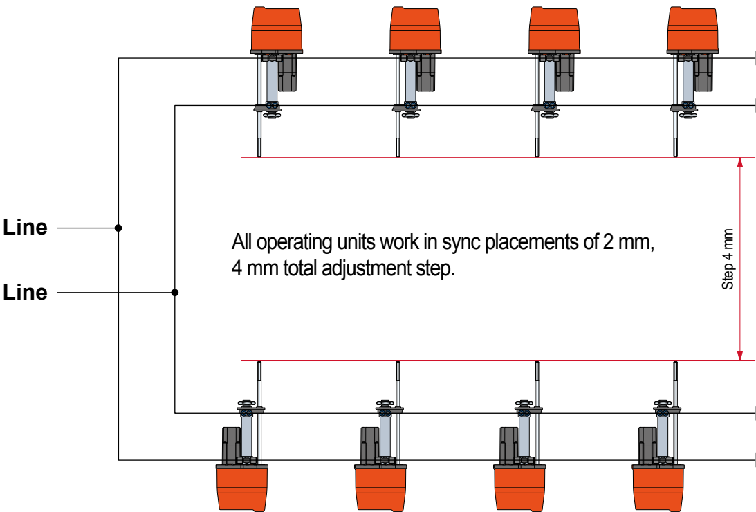
Assembly drawing 1
