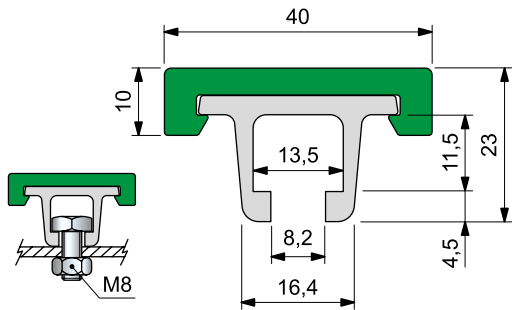
Assembly with M8 hexagon bolt
