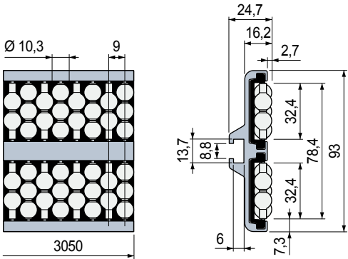
Pearl roller side guide
