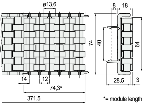
Sideflexing
