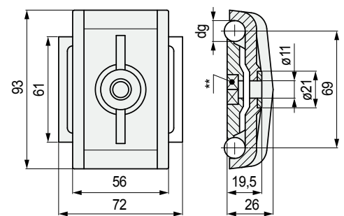
Double guide-rail clamp
