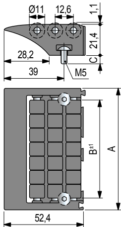
End transfer module (with lip)
