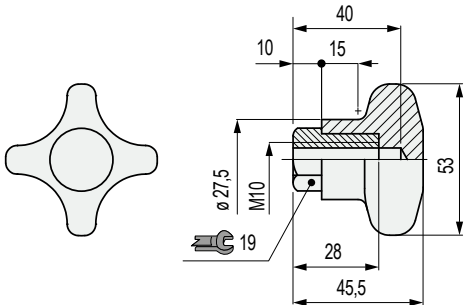
Tightening knob
