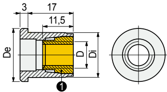
Tube dimensions 1 Expansion cone
