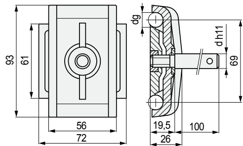
Double guide-rail clamp
