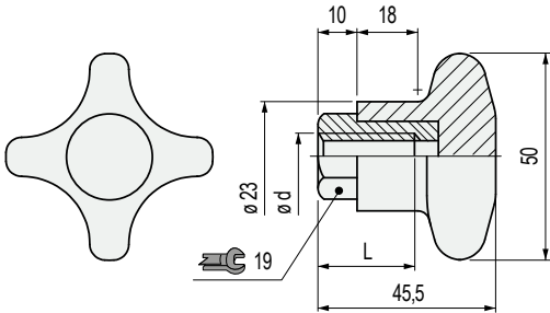
Tightening knob
