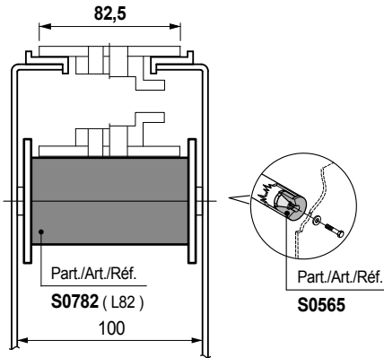
Chain width 82,5 mm (K325) / Pitch 85 mm
