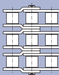
Offset link double
