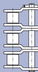
Offset link with splint
