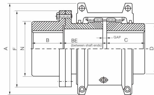
SFS(Half Space)Type
