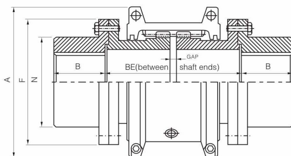
SAS(Full Space)Type
